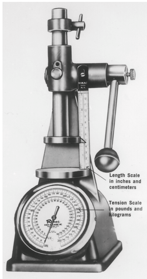
Figure 4.4.5.2.1-1(a) Rimac Spring Tester without gearbox modification (Contact the CBM if a Shop Drawing for gear modification is desired).
