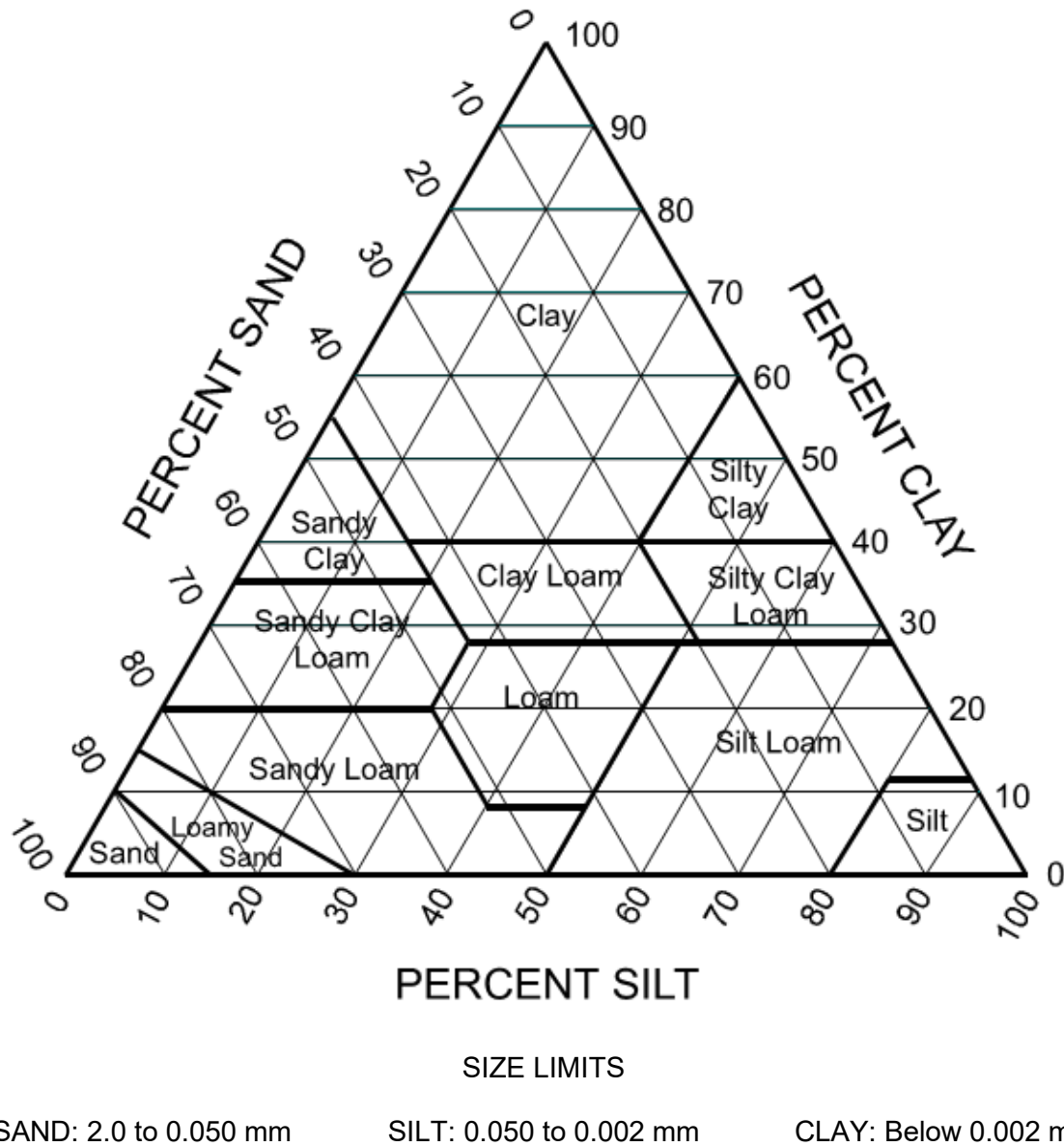
Figure A.5.1-1 USDA/NRCS Textural Classification Diagram
