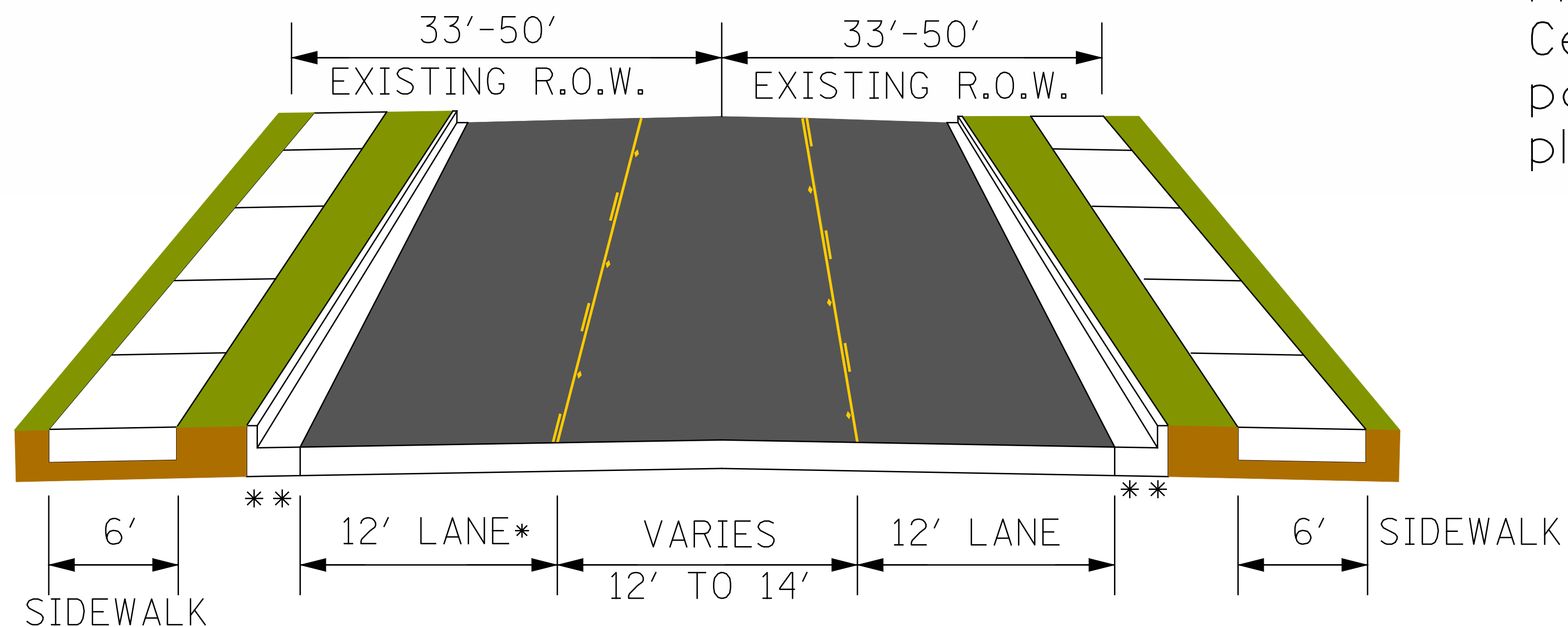
IL Route 31 Prime Parkway to IL Route 120 Existing Typical Section
