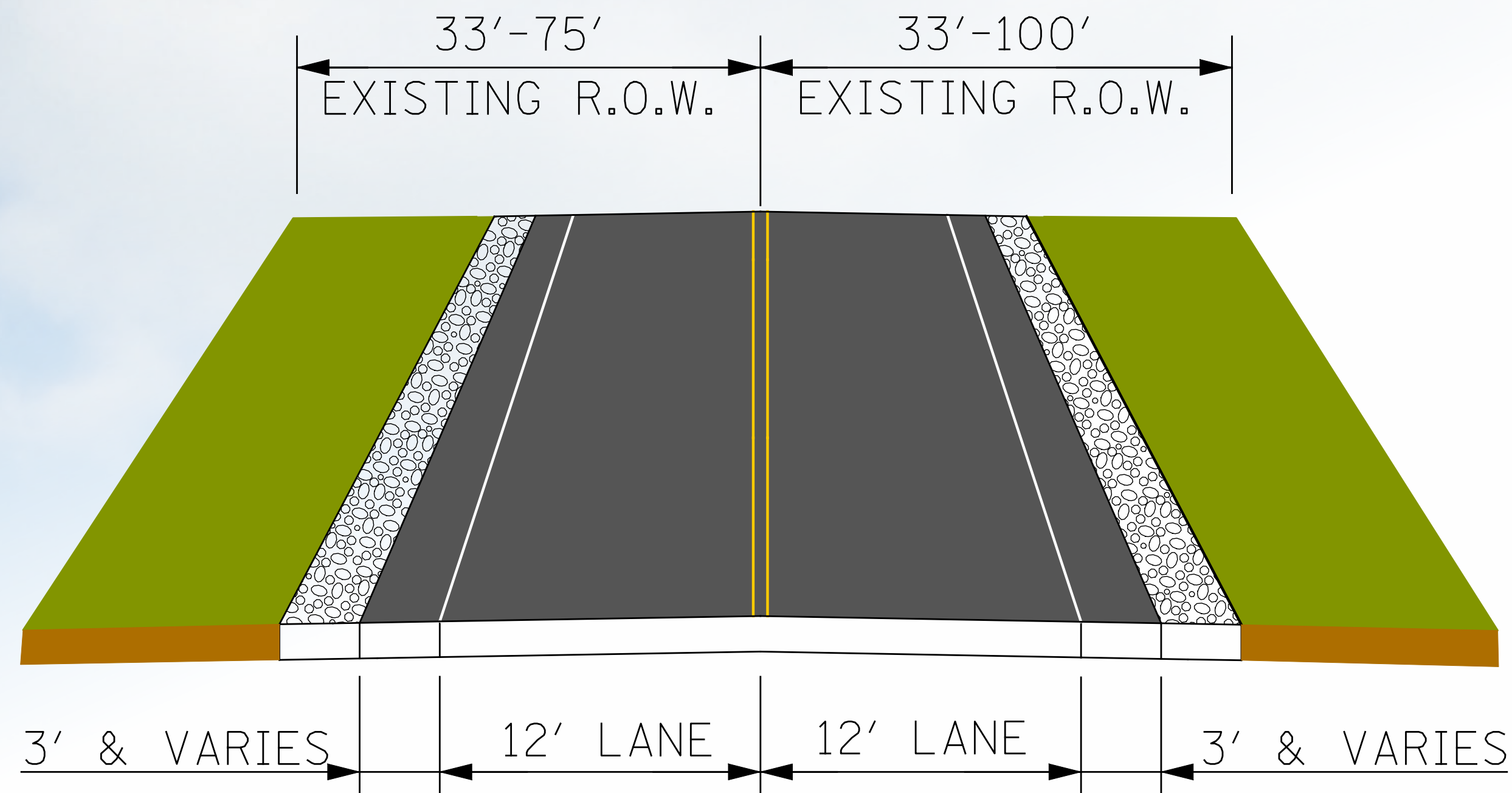
IL Route 31 IL Route 176 to Prime Parkway Existing Typical Section
